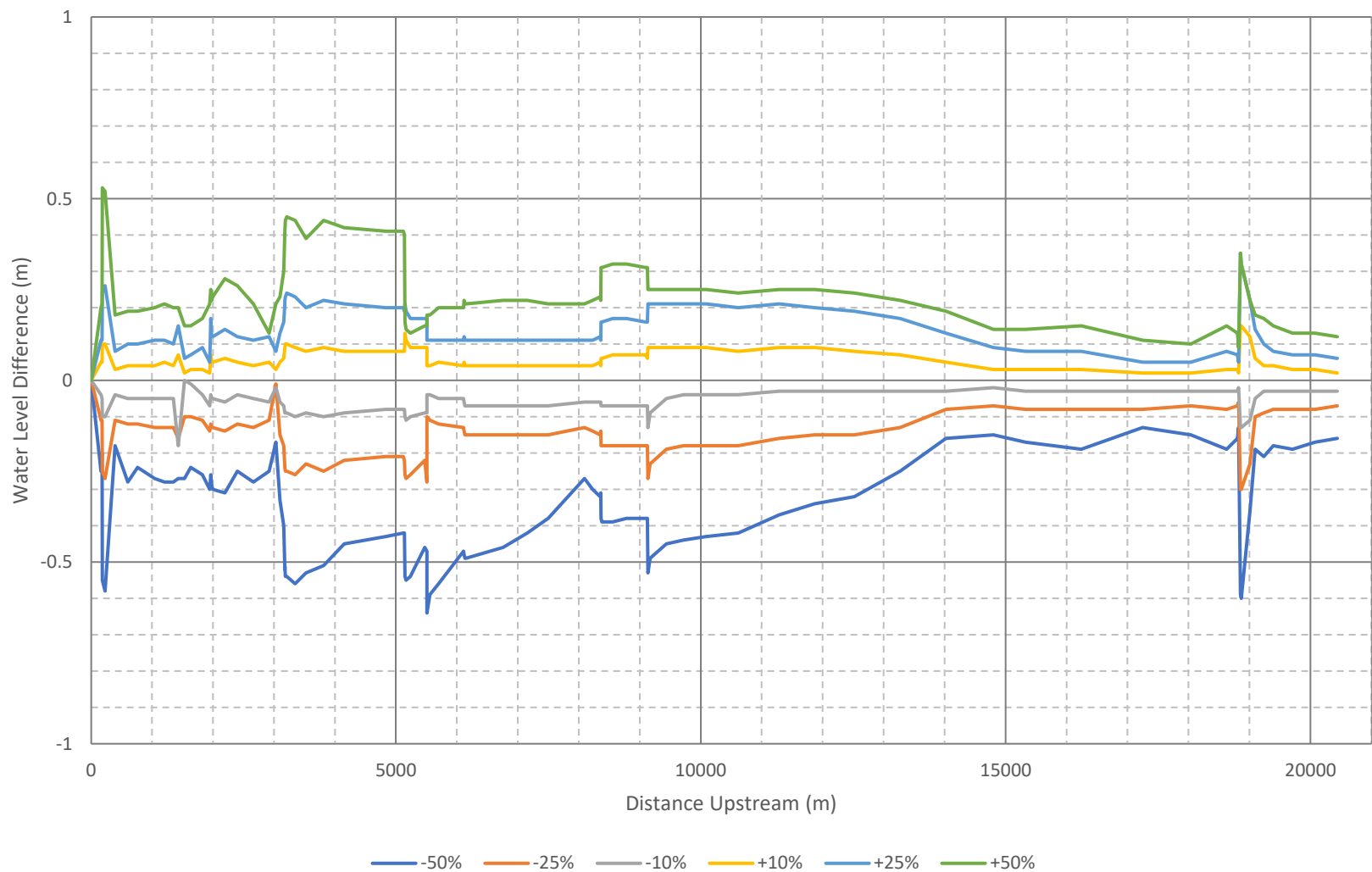
Figure 19 Sensitivity analysis of computed water level.
