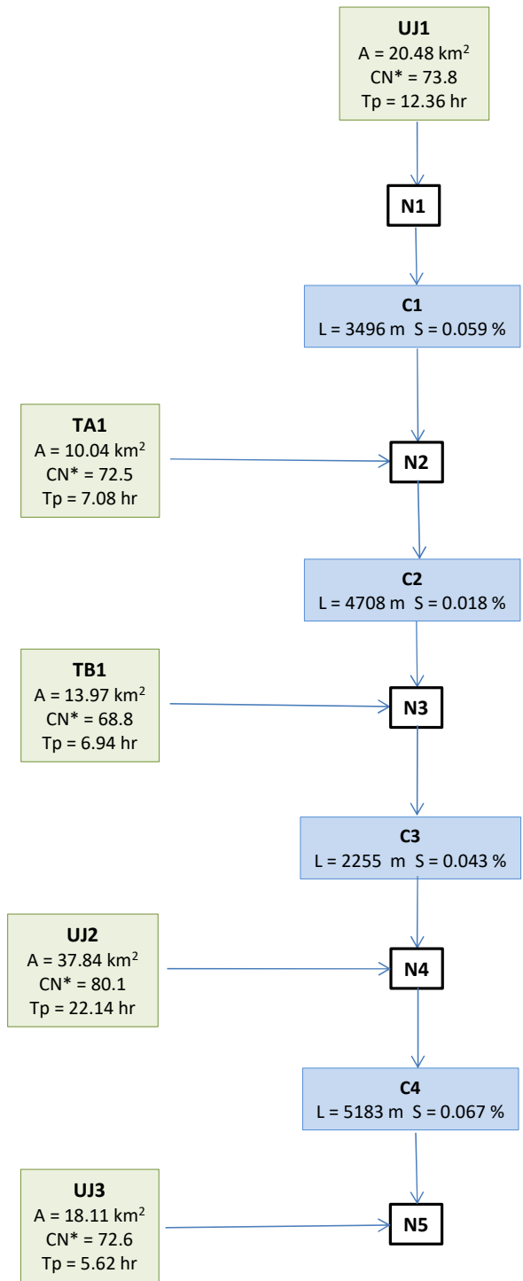
Figure 8 SWMHYMO Flow Chart
