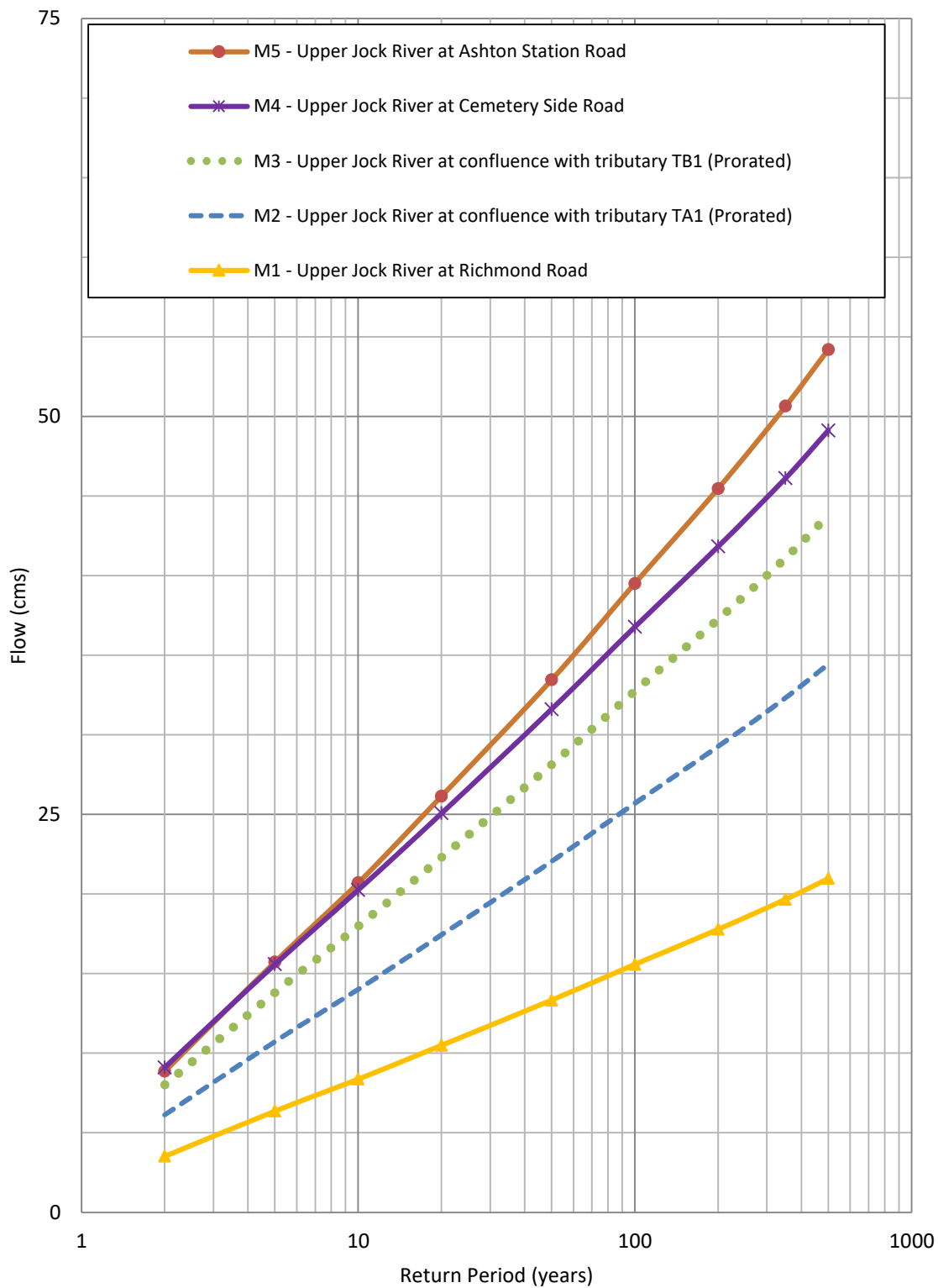
Figure 14 Estimated flows along Upper Jock River
