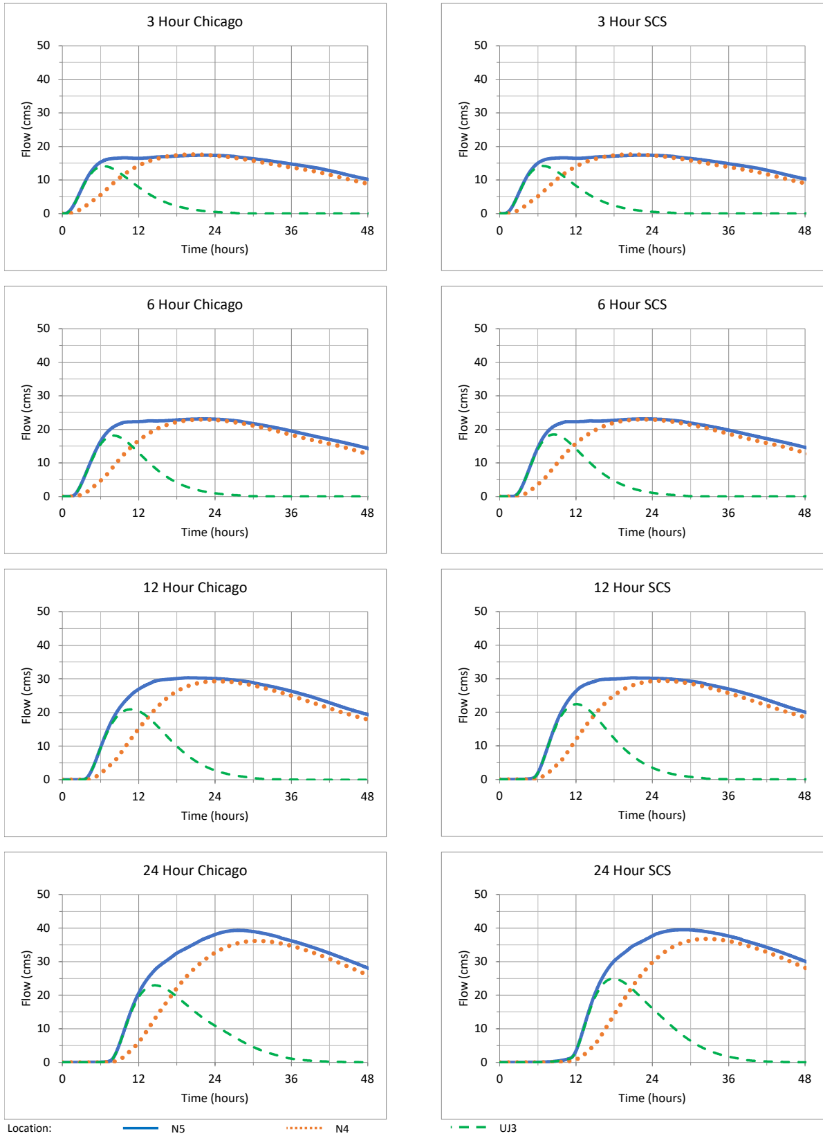
Figure 12 SWMHYMO generated 100 Year flows.
