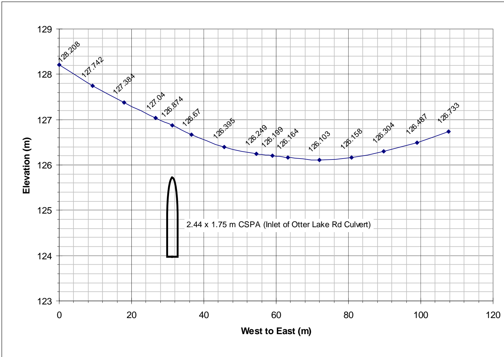
Figure 7: Otter Lake Road Profile and Culvert
